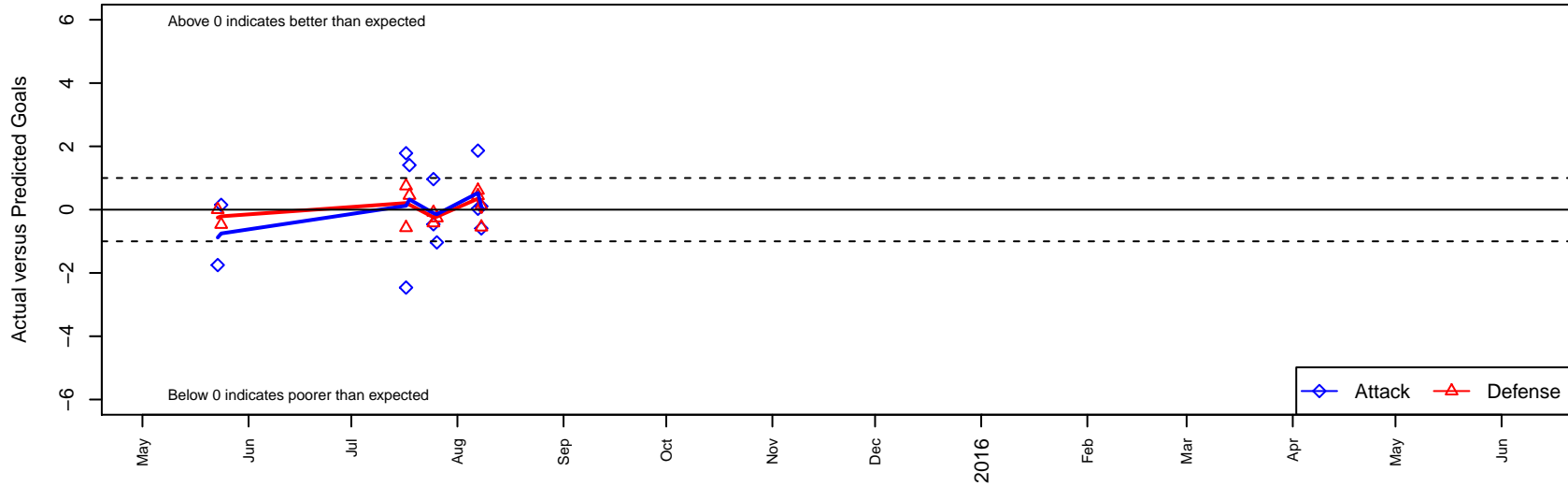
Atletico Santa Rosa Leones B98 Dots are actual minus expected GF (blue circles) and GA (red triangles). Blue line is smoothed change in attack strength. Red is smoothed change in defense strength.
